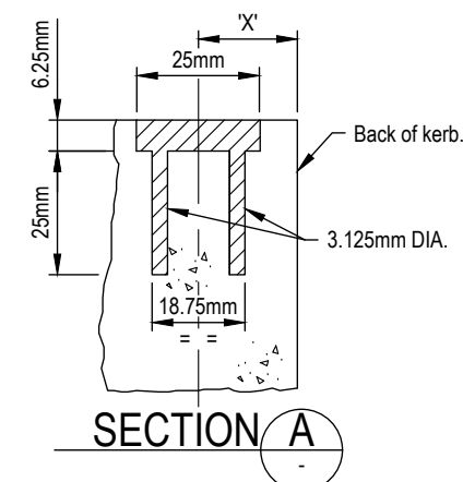
BRASS or STAINLESS STEEL SERVICE CONDUIT MARKER and VALVE MARKER DISC
