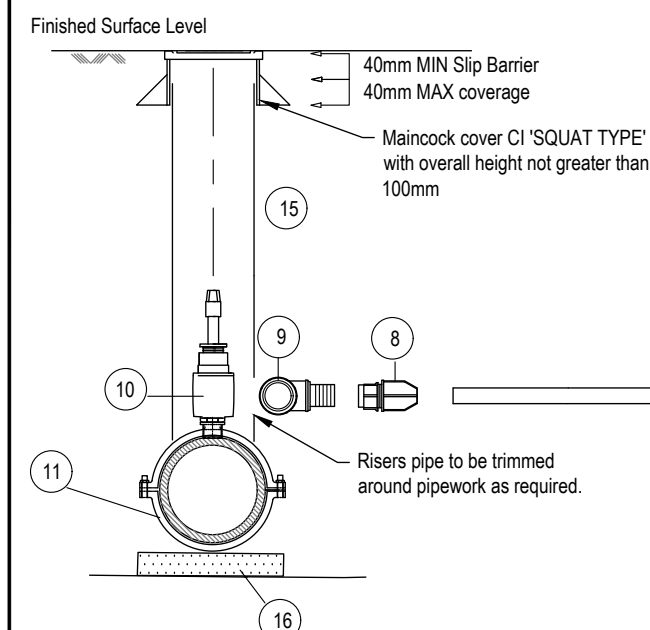
WATER MAIN CONNECTION DETAIL ELEVATION
