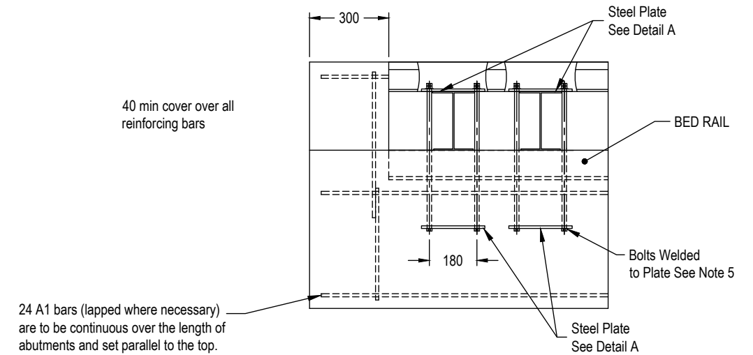
ABUTMENT DETAIL 2 SCALE 1:20
