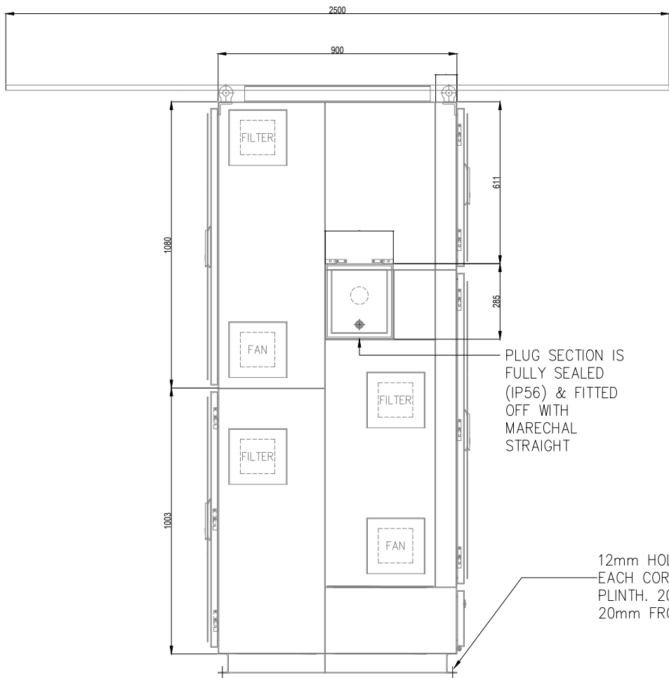
LH SIDE VIEW
