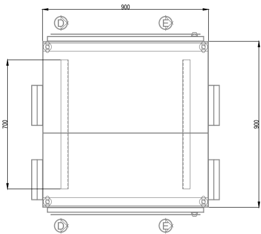
TOP VIEW (ROOF REMOVED)
