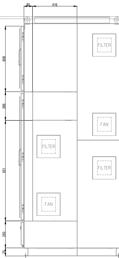
RH SIDE VIEW
