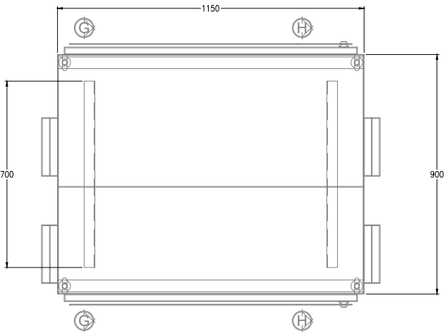
TOP VIEW (ROOF REMOVED)
