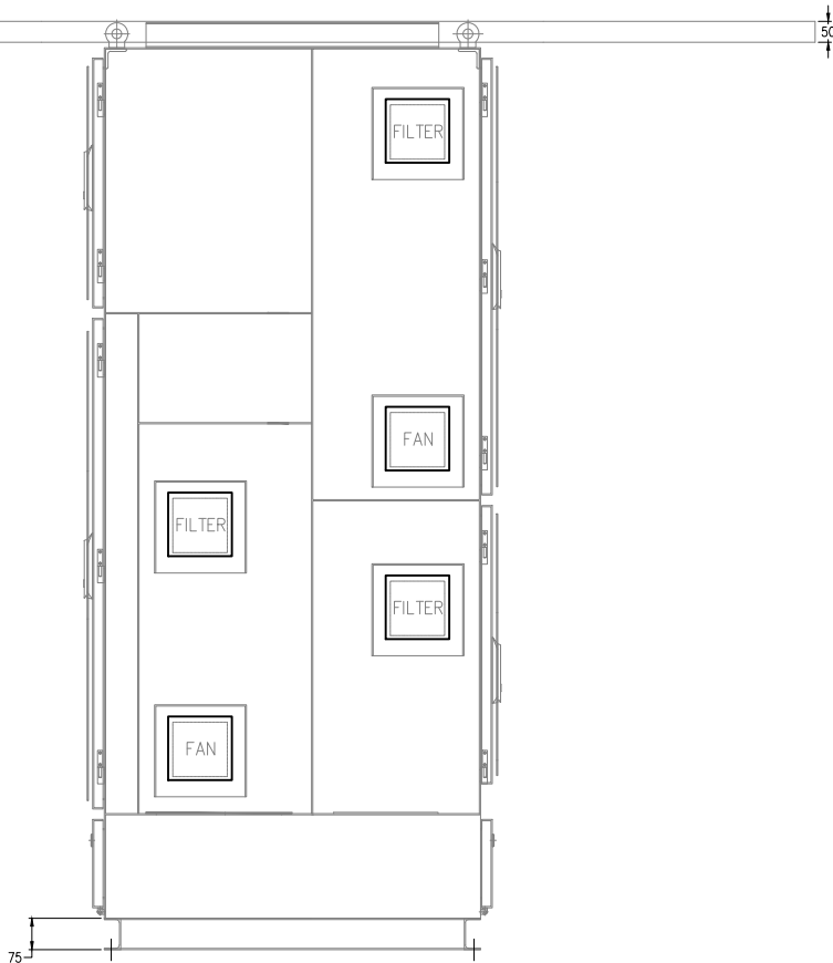
RH SIDE VIEW
