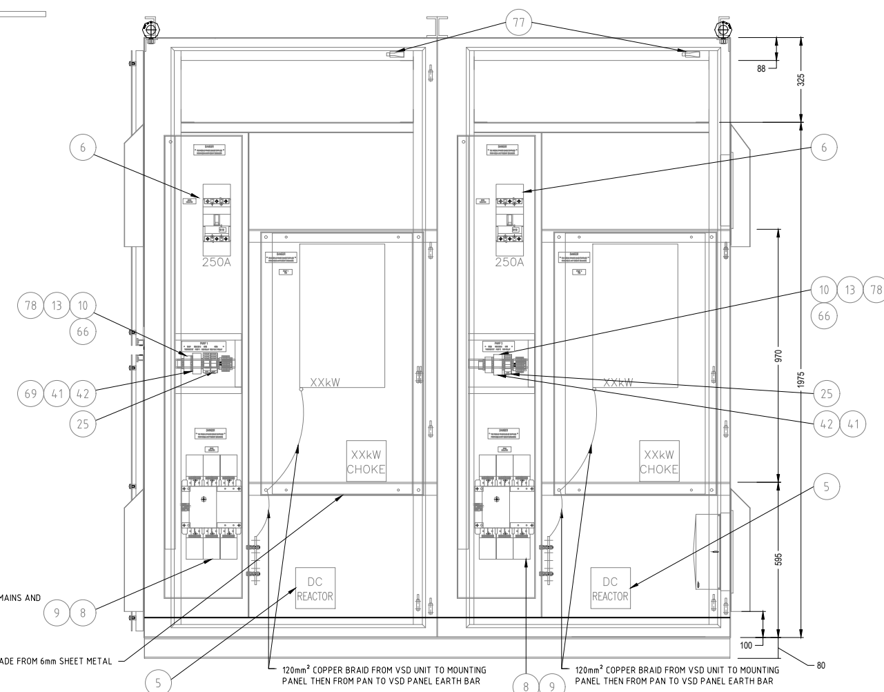
REAR VIEW (OUTER DOORS REMOVED SHOWING GEAR TRAY)
